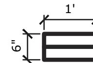
6" x 12" Filler Stone – Double Part No.: BFL36126D
