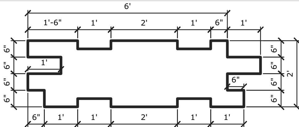
2' Country Ledge Form Liner Part No.: BFL3624 Patent No. 5,885,502
